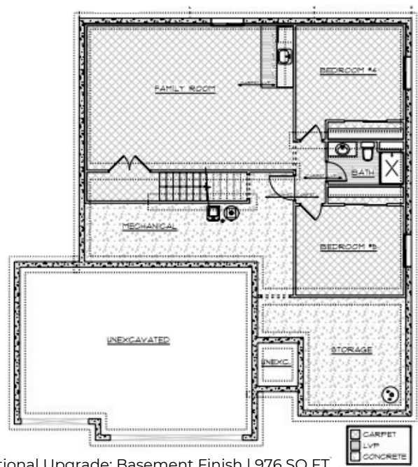
Optional Upgrade: Basement Finish | 976 SQ FT Living Space | 2 Bed | 1 Bath | Optional Wet Bar
